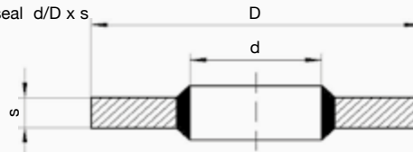
Dowty seal d/D x s
